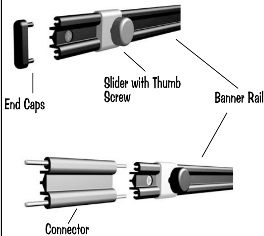
BT 1002 Connector
